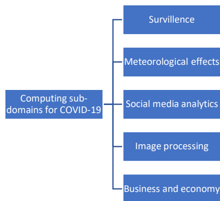
FIGURE 1. Categorization of methods that study coronavirus
